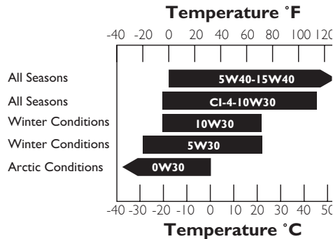
Fig.7.I. Recommended SAE Oil Viscosity Grades v.s. Ambient Temperatures
