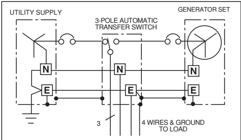
Fig. 10.2. 3 phase 4 wire connection 3 pole switched
