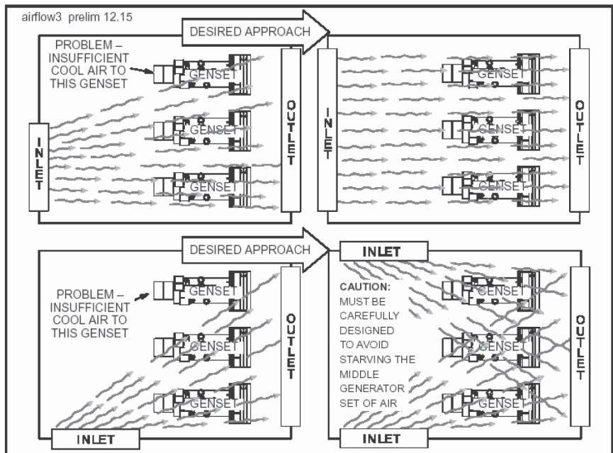
Figure 6.5. Multiple GenSet Air Ventilation
